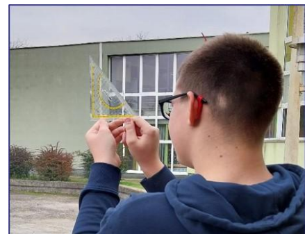
Figure 30 . Measuring tree height using an isosceles right triangle
